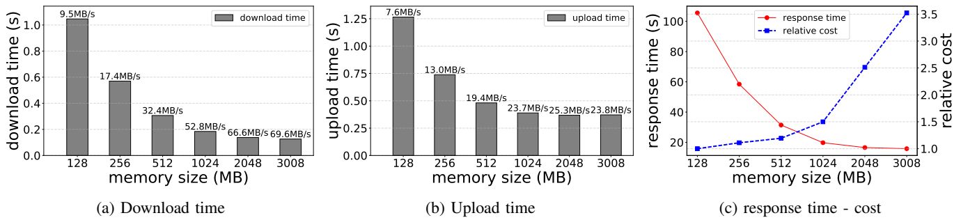
Fig. 4: The impact of function’s configured memory size to the network performance and cost
