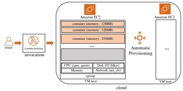
Fig. 1: Procedure of function invocation (AWS Lambda)
