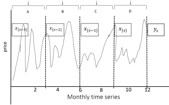
Fig. 1 SARIMA example
